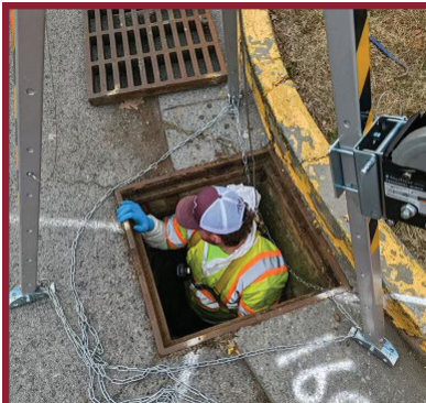
MANHOLE INSPECTION
